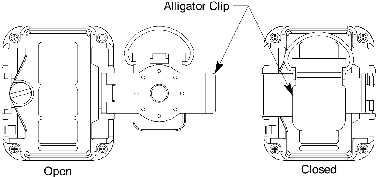
Figure 3: Alligator Clip
