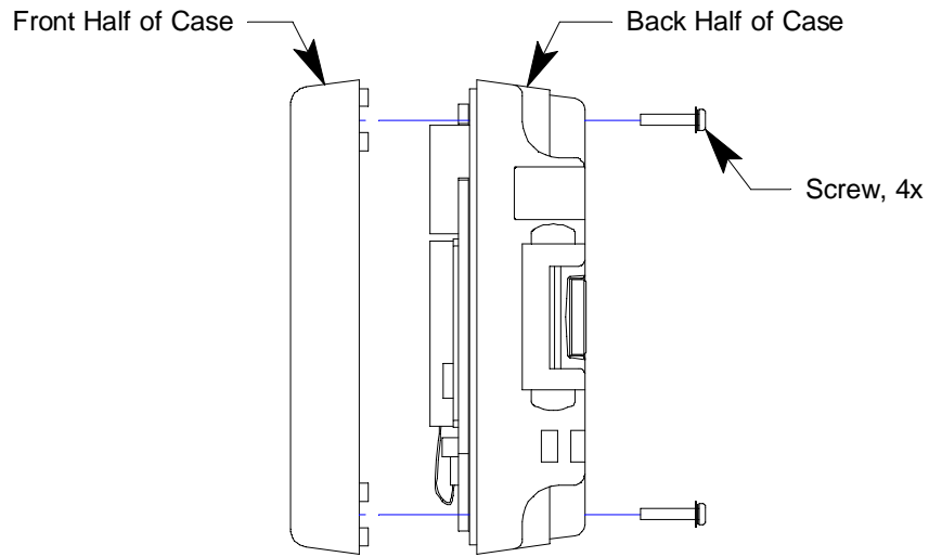
Figure 17: Case Separation
