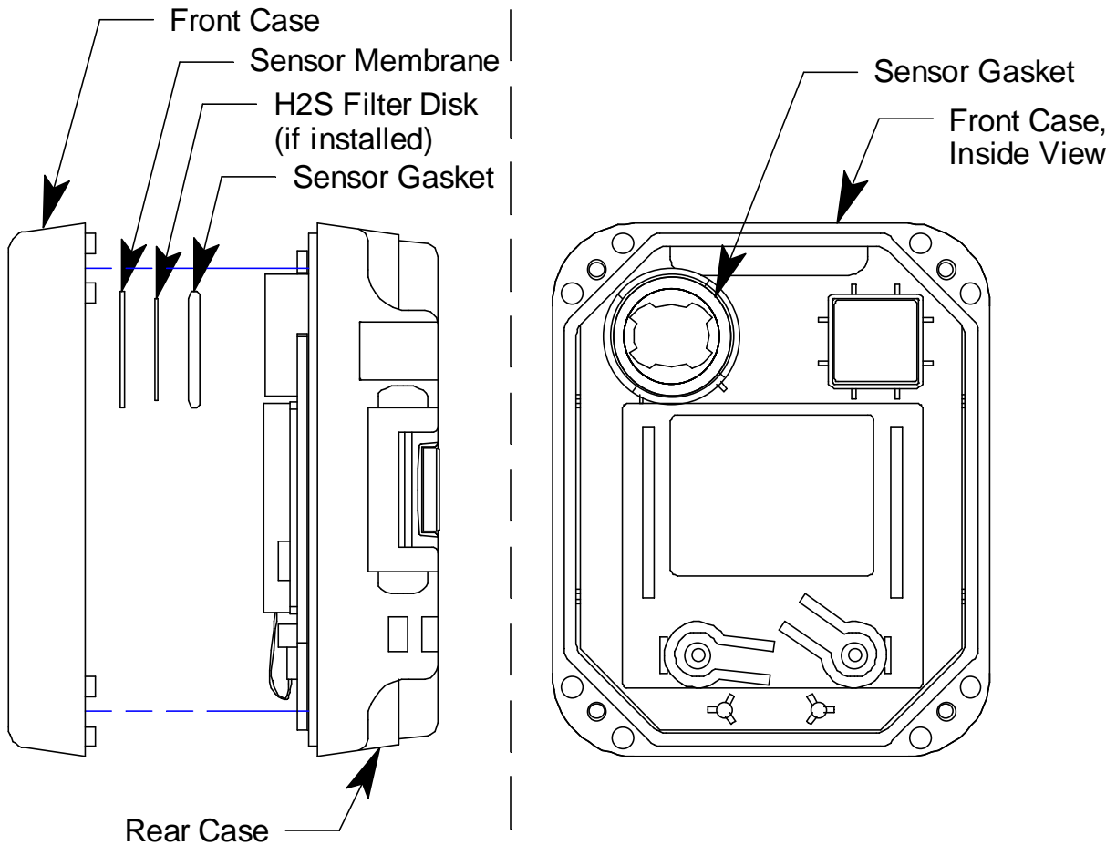
Figure 18: Replacing the Sensor Membrane and H2S Filter Disk
